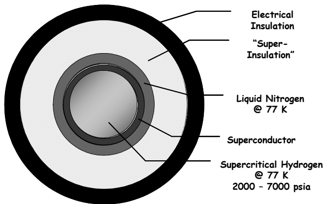
Fig. 2. Hybrid SuperCable with liquid nitrogen as the primary cryogen and high pressure, low temperature hydrogen as the chemical energy transfer fluid. The scale is roughly that of Fig. 1.
