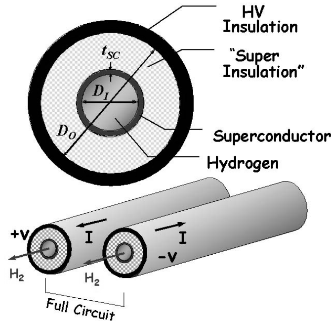
Fig. 1. SuperCable cross-section schematic (roughly to scale) for one pole of a bipolar circuit.
