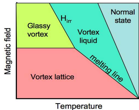
Figure 5 Schematic vortex phase diagram of a high-temperature superconductor. ( H_{\text{irr}} = irreversibility field, discussed later)
